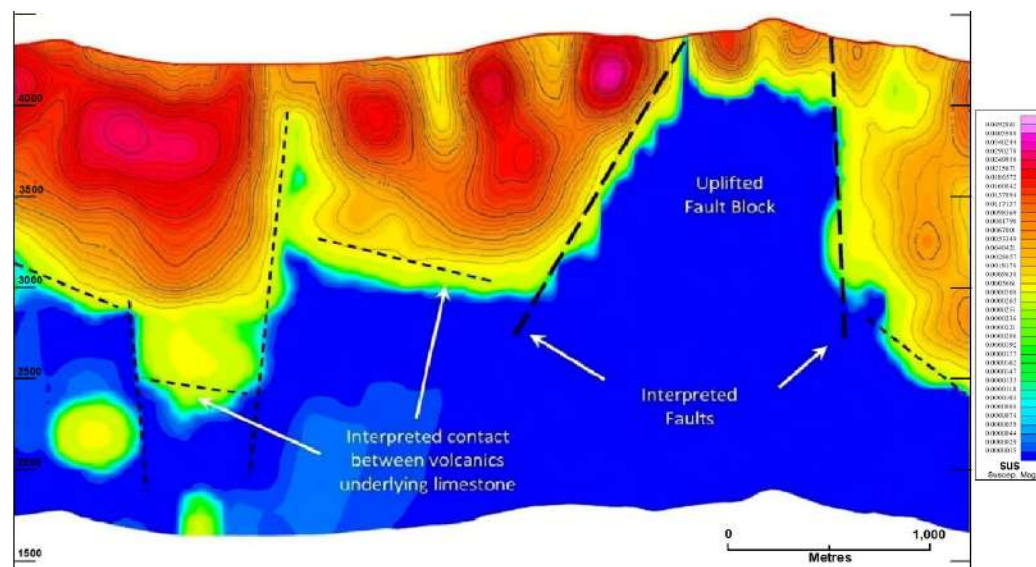
Gris Zone : Cross-section of inverted magnetic susceptibility uplifted limestones (blue) bounded by volcanic rocks (yellow/magenta).
