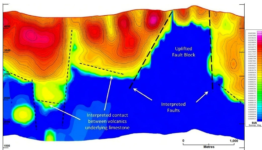
Priority Drill Target Area: Cross-section of the inverted magnetic susceptibility in the historical Chaparro & Gaspar galena mines area with uplifted limestones (blue) bounded by volcanic rocks (yellow/magenta).
